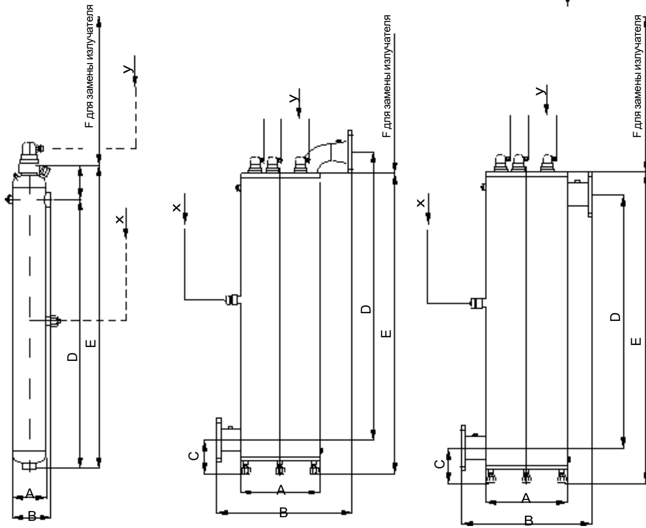
80W80/11 N - 100W100/11 N
